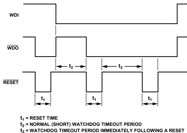
Figure 16. Watchdog Timeout Period and Reset Active Time
