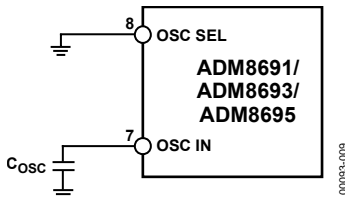
Figure 18. External Capacitor
