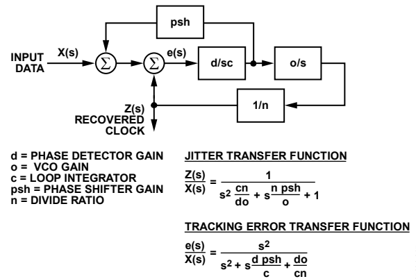
Figure 17. PLL/DLL Architecture
