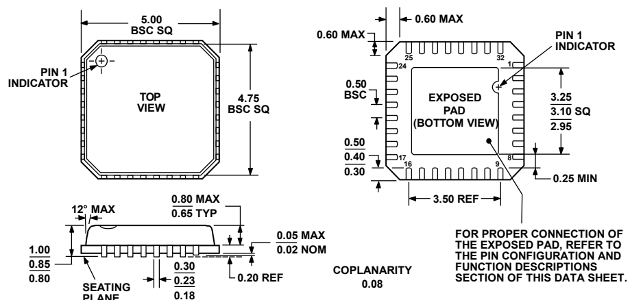
Figure 30. 32-Lead Frame Chip Scale Package [LFCSP_VQ]
