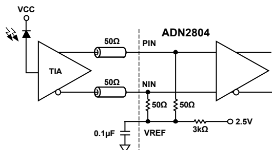
Figure 27. DC-Coupled Application
