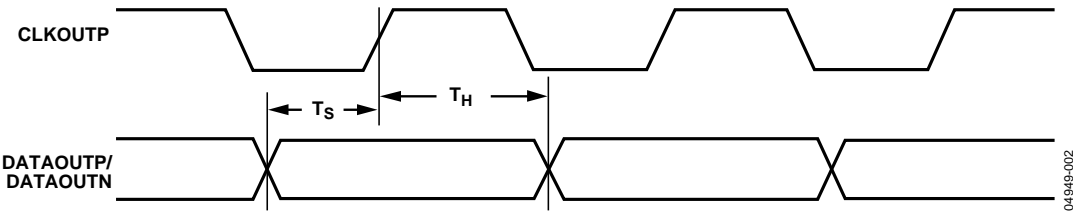
Figure 2. Output Timing
