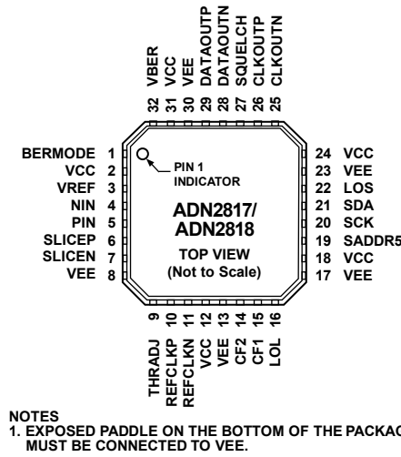
Figure 5. Pin Configuration
