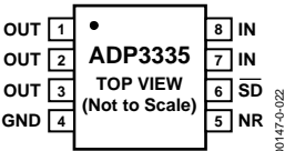
Figure 3. 8-Lead MSOP
