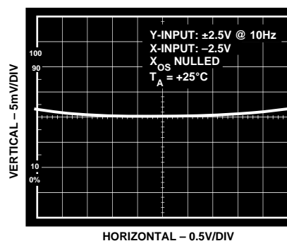
Figure 12. Y-Input Nonlinearity @ X = -2.5\text{ V}
