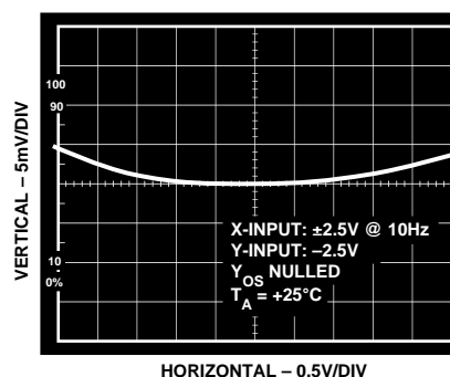
Figure 10. X-Input Nonlinearity @ Y = -2.5\text{ V}
