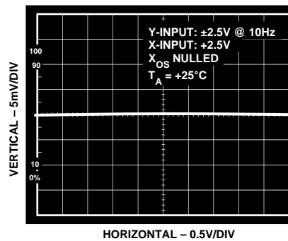
Figure 11. Y-Input Nonlinearity @ X = +2.5\text{ V}
