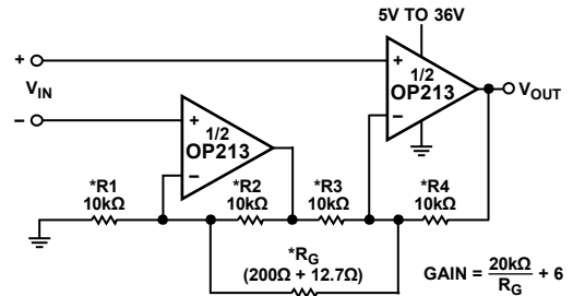
Figure 45. Ultralow Noise, Single Supply Instrumentation Amplifier
