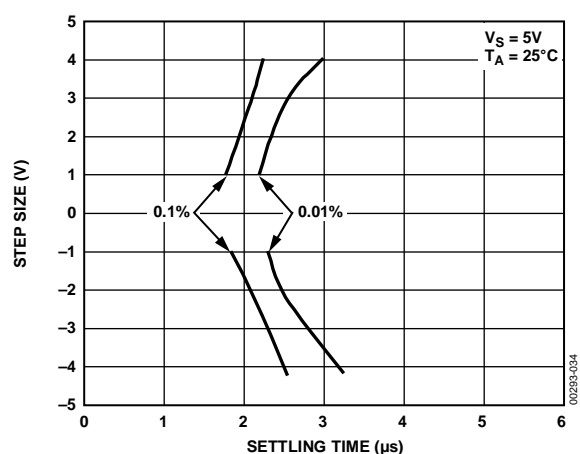
Figure 34. Step Size vs. Settling Time
