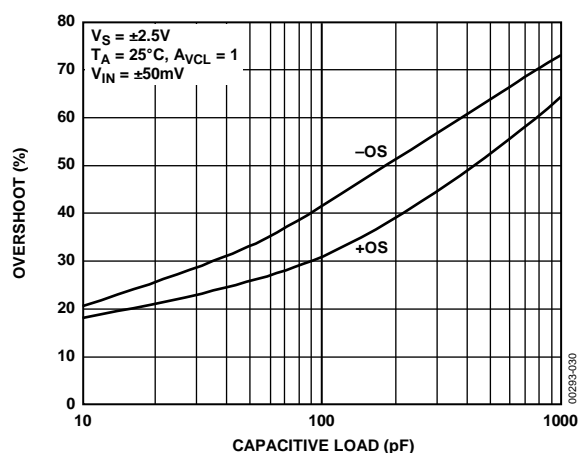
Figure 30. Small Signal Overshoot vs. Capacitive Load
