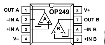
Figure 1. 8-Lead Cerdip (Q-8) and 8-Lead PDIP (N-8)
