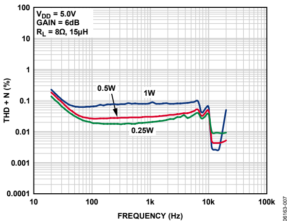
Figure 6. THD + N vs. Frequency, V_{DD} = 5.0\ \text{V} , A_V = 6\ \text{dB} , R_L = 8\ \Omega
