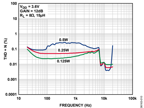
Figure 9. THD + N vs. Frequency, V_{DD} = 3.6\ \text{V} , A_V = 12\ \text{dB} , R_L = 8\ \Omega
