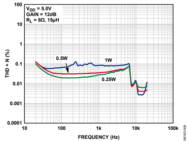
Figure 7. THD + N vs. Frequency, V_{DD} = 5.0\ \text{V} , A_V = 12\ \text{dB} , R_L = 8\ \Omega
