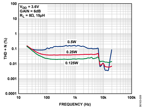
Figure 8. THD + N vs. Frequency, V_{DD} = 3.6\ \text{V} , A_V = 6\ \text{dB} , R_L = 8\ \Omega
