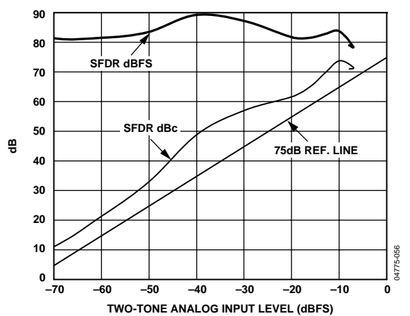
Figure 21. Two-Tone IMD Performance vs. Input Drive Level (69.1 MHz and 70.1 MHz; f_s = 65 \text{ MSPS} ( -65 \text{ Grade} ); F_1, F_2 Levels Equal)
