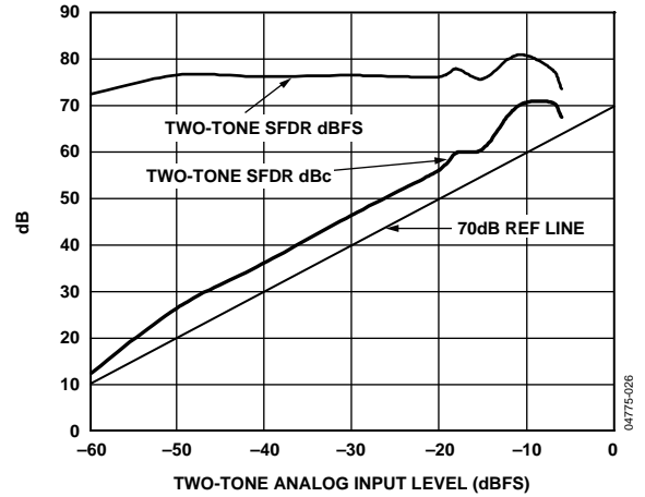
Figure 19. Two-Tone IMD Performance vs. Input Drive Level (69.1 MHz and 70.1 MHz; f_s = 105 \text{ MSPS} ( -105 \text{ Grade} ); F_1, F_2 Levels Equal)
