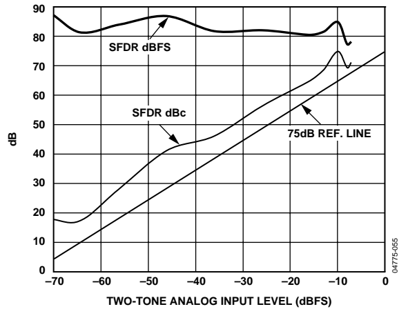
Figure 20. Two-Tone IMD Performance vs. Input Drive Level (69.1 MHz and 70.1 MHz; f_s = 80 \text{ MSPS} ( -80 \text{ Grade} ); F_1, F_2 Levels Equal)
