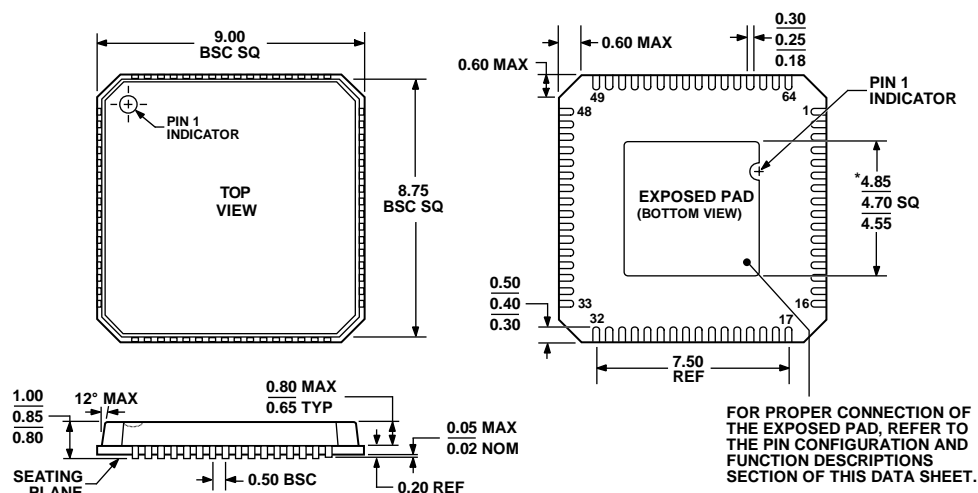
Figure 60. 64-Lead Lead Frame Chip Scale Package [LFCSP_VQ] 9 mm × 9 mm Body, Very Thin Quad (CP-64-1) Dimensions shown in millimeters
