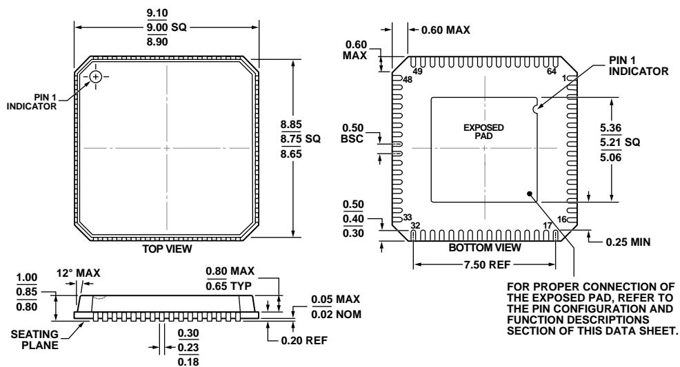
Figure 60. 64-Lead Lead Frame Chip Scale Package [LFCSP_VQ] 9 mm × 9 mm Body, Very Thin Quad (CP-64-1) Dimensions shown in millimeters
