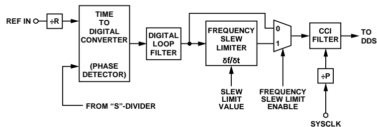
Figure 47. Frequency Slew Limiter Rev. B | Page 37 of 76
