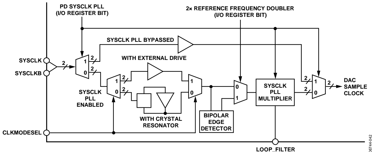
Figure 42. System Clock Generator Block Diagram Rev. B | Page 33 of 76
