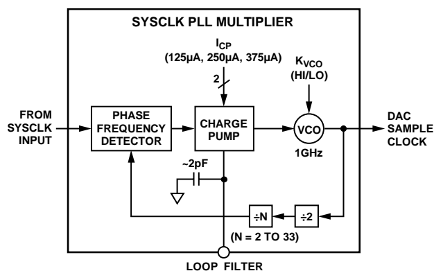
Figure 43. Block Diagram of the SYSCLK PLL
