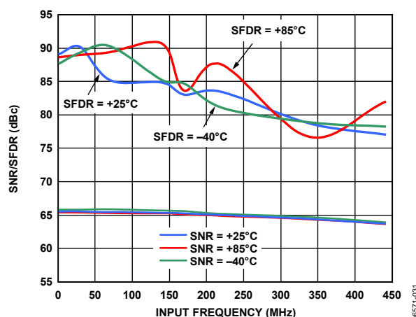
Figure 31. AD9627-150 Single-Tone SNR/SFDR vs. Input Frequency ( f_{IN} ) and Temperature with 1 V p-p Full Scale
