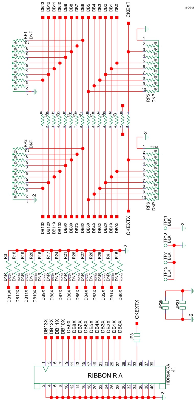
Figure 92. Digital Inputs
