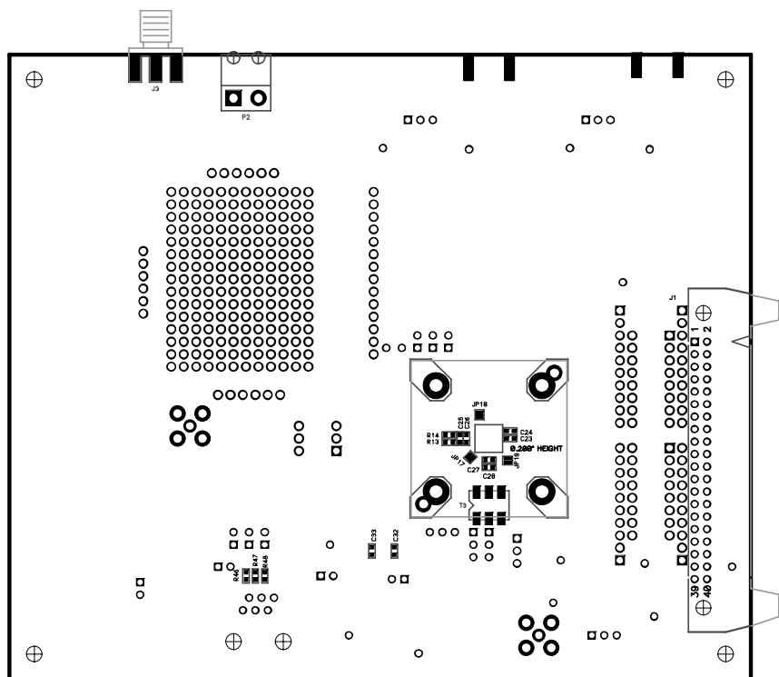
Figure 98. Assembly—Secondary Side
