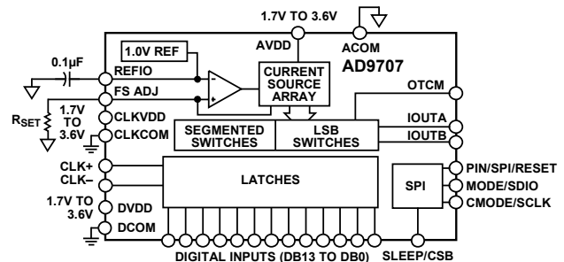
Figure 1. AD9707
