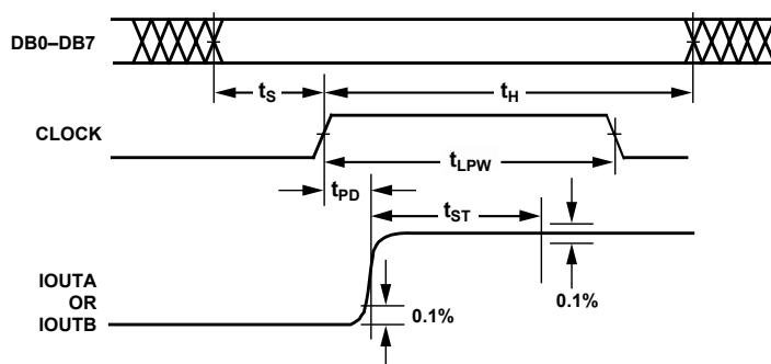
Figure 2. Timing Diagram
