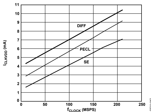
Figure 24. I_{CLKVDD} vs. f_{CLOCK} and Clock Mode
