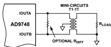
Figure 25. Differential Output Using a Transformer
