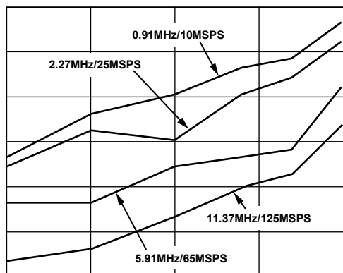
Figure 29. Single-Tone SFDR vs. A_{OUT} @ f_{OUT} = f_{CLK}/11
