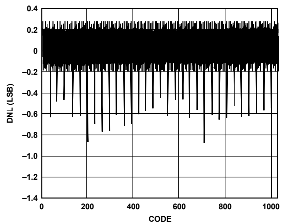
Figure 51. Typical DNL
