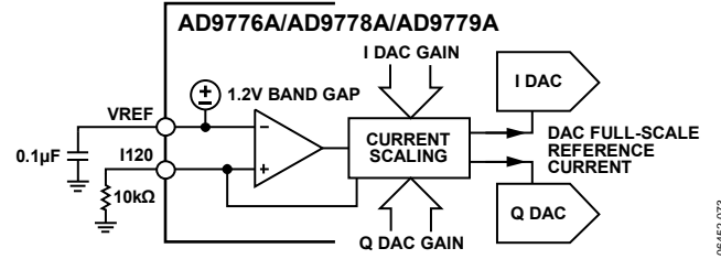
Figure 75. Reference Circuitry
