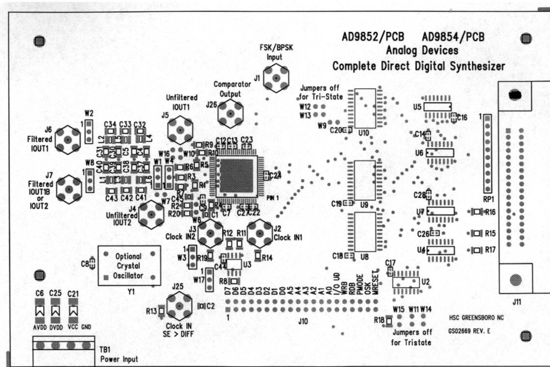
Figure 63. Assembly Drawing
