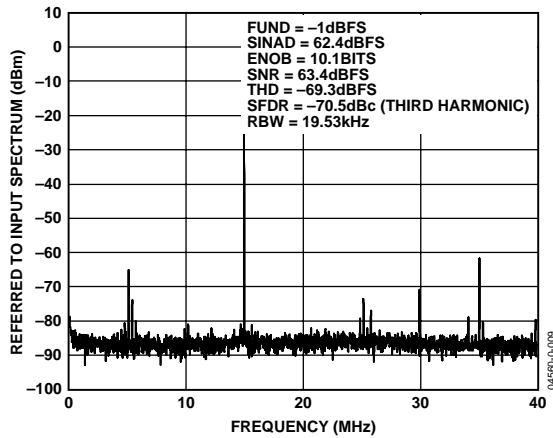
Figure 9. Spectral Plot with 4k FFT of Input Sinusoid with RxPGA = 0 dB and P_{\text{IN}} = 9 \text{ dBm}
