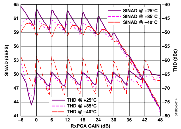
Figure 14. SINAD/THD Performance vs. RxPGA Gain and Temperature ( f_{\text{IN}} = 10 \text{ MHz} )
