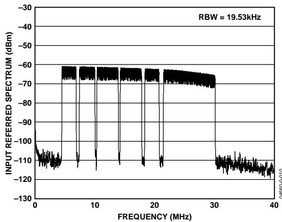
Figure 10. Spectral Plot with 4K FFT of 111-Carrier DMT Signal with \text{PAR} = 11 \text{ dB} , P_{\text{IN}} = -33.7 \text{ dBm} , LPF's f_{-3\text{dB}} = 32 \text{ MHz} and RxPGA = 36 dB
