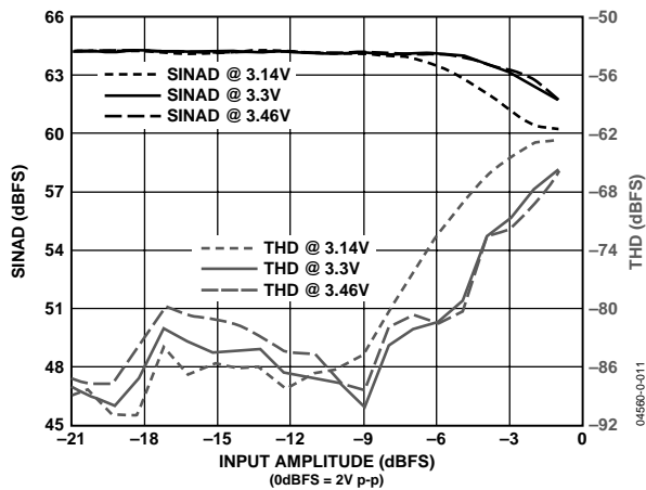
Figure 11. SINAD and THD vs. Input Amplitude and Supply ( f_{\text{IN}} = 8 \text{ MHz} , LPF f_{-3\text{dB}} = 26 \text{ MHz} ; RxPGA = 0 dB)
