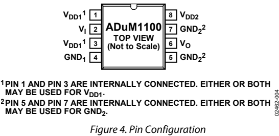
Figure 4. Pin Configuration
