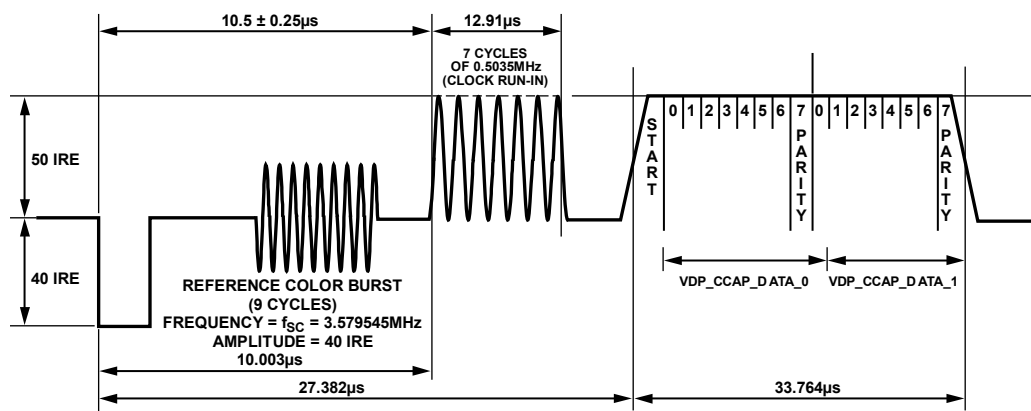
Figure 44. CCAP Waveform and Decoded Data Correlation
