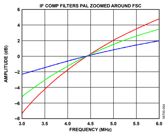
Figure 29. PAL IF Filter Compensation
