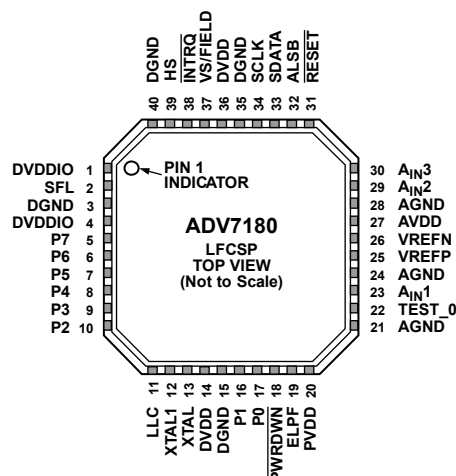
Figure 6. 40-Lead LFCSP Pin Configuration
