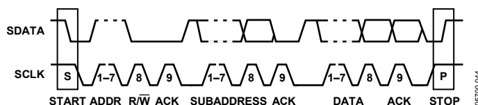
Figure 47. Bus Data Transfer
