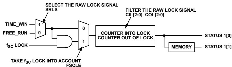
Figure 15. Lock Related Signal Path
