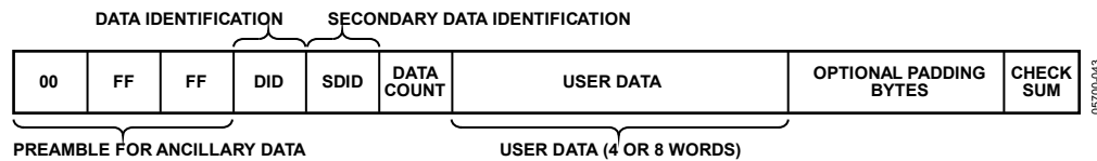
Figure 46. Gemstar- and CCAP-Embedded Data Packet (Generic)
