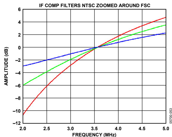
Figure 28. NTSC IF Filter Compensation
