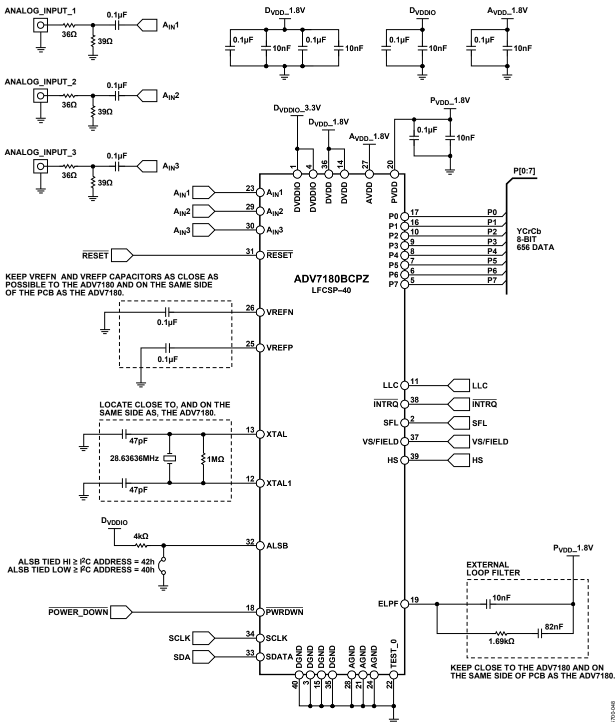
Figure 52. 40-Lead LFCSP Typical Connection Diagram
