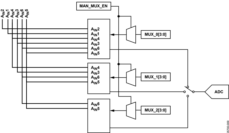
Figure 8. 64-Lead LQFP Internal Pin Connections
