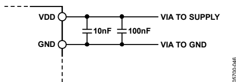
Figure 50. Recommended Power Supply Decoupling
