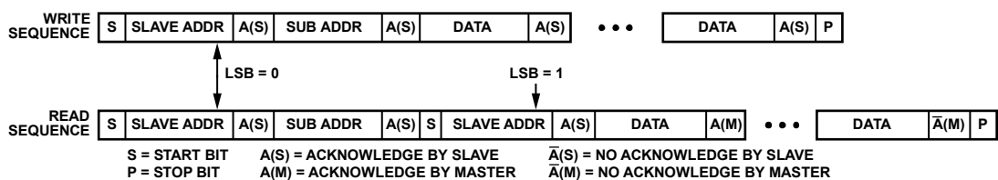
Figure 48. Read and Write Sequence
