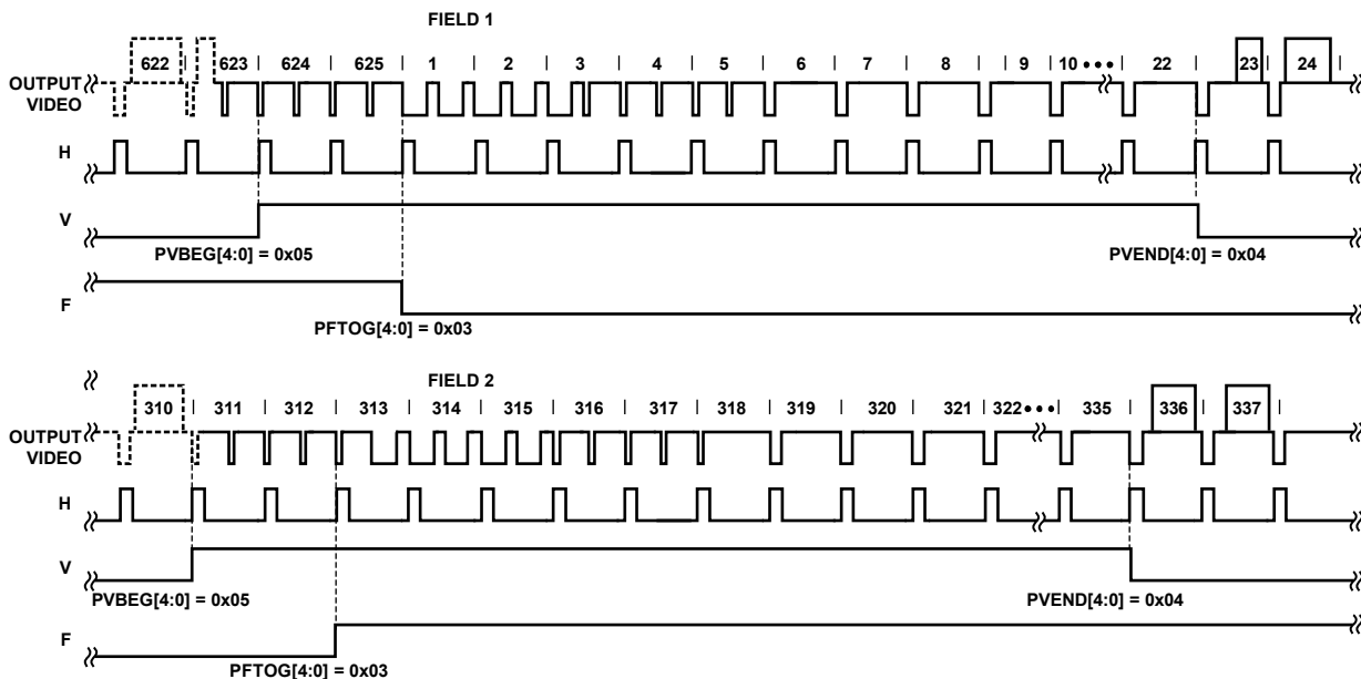
Figure 37. PAL Default, ITU-R BT.656 (the Polarity of H, V, and F is Embedded in the Data)
