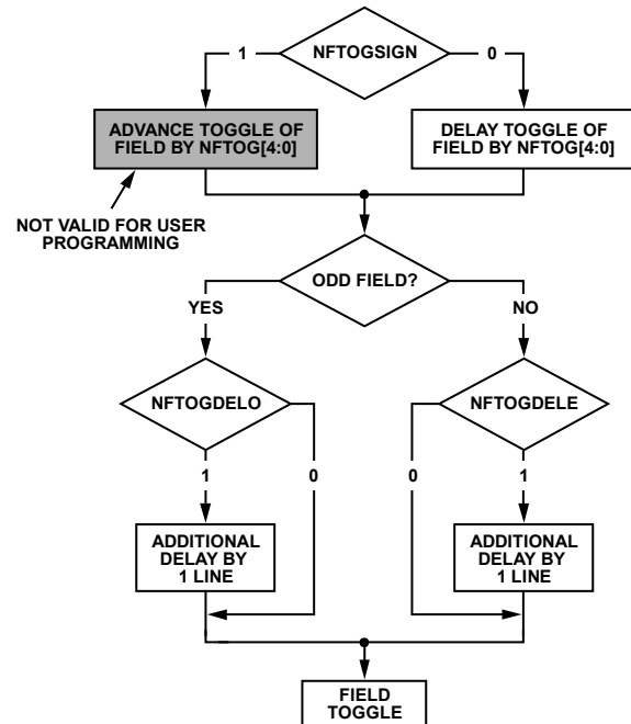
Figure 36. NTSC FIELD Toggle
