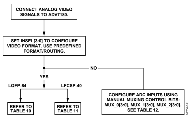
Figure 10. Signal Routing Options
