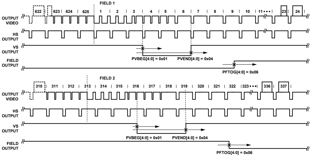
Figure 38. PAL Typical VS/FIELD Positions Using Register Writes Shown in Table 63
