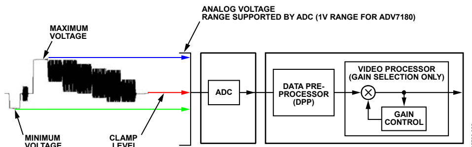
Figure 24. Gain Control Overview
