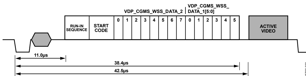
Figure 42. WSS Waveform
