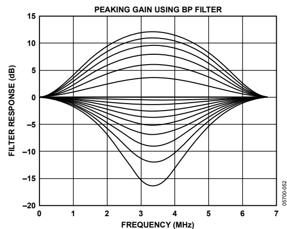
Figure 27. Peaking Filter Responses
