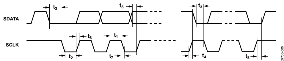
Figure 4. I²C Timing
