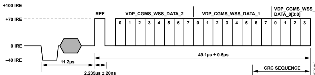
Figure 43. CGMS Waveform
