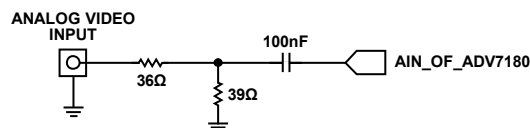
Figure 23. Input Voltage Divider Network
