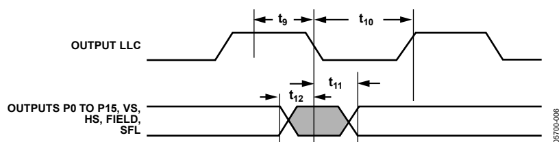
Figure 5. Pixel Port and Control Output Timing
