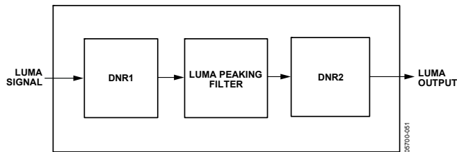
Figure 26. DNR and Peaking Block Diagram
