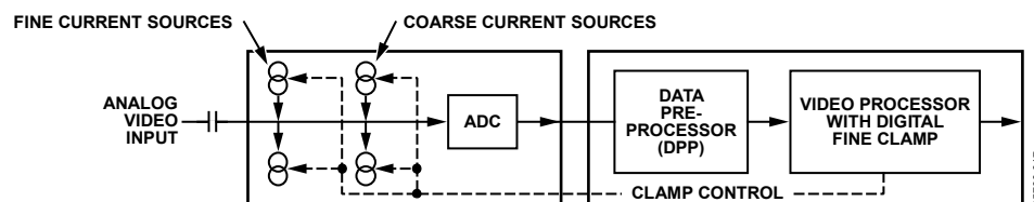
Figure 16. Clamping Overview
