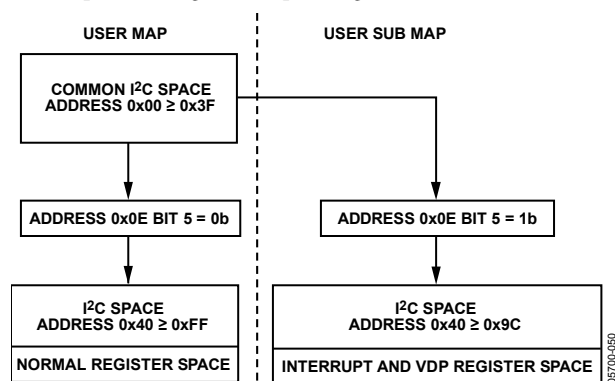
Figure 49. Register Access—User Map and User Sub Map
