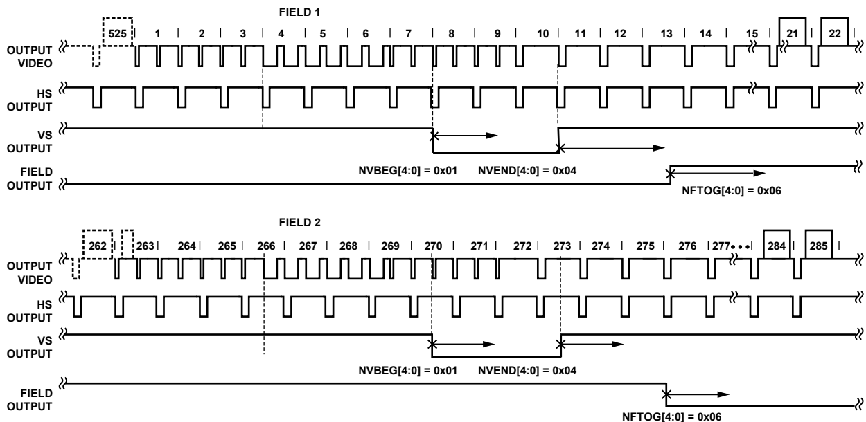
Figure 33. NTSC Typical VSYNC/FIELD Positions Using Register Writes in Table 62
