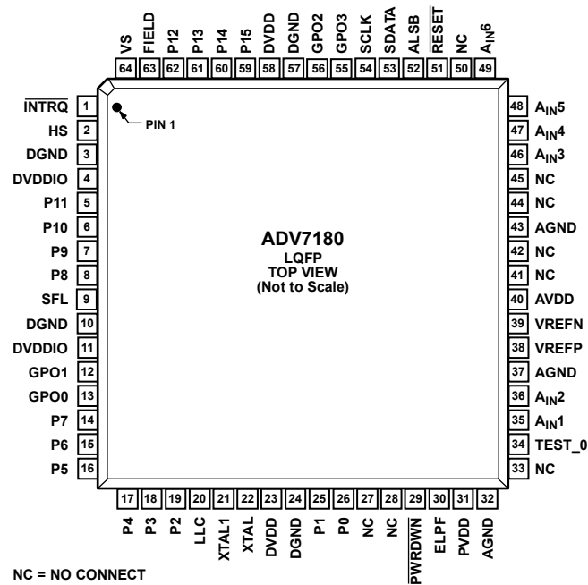
Figure 7. 64-Lead LQFP Pin Configuration
