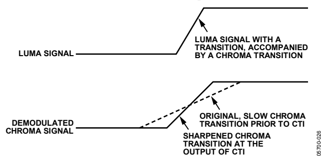
Figure 25. CTI Luma/Chroma Transition
