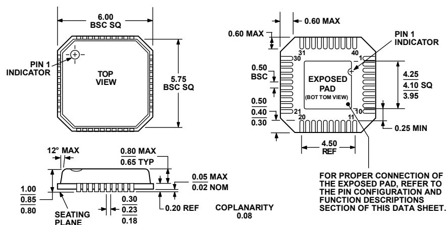
Figure 54. 40-Lead Lead Frame Chip Scale Package [LFCSP_VQ] 6 mm x 6 mm Body, Very Thin Quad (CP-40-1) Dimensions shown in millimeters
