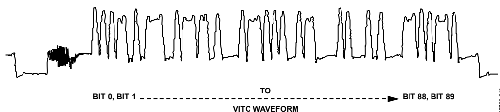
Figure 45. VITC Waveform and Decoded Data Correlation
