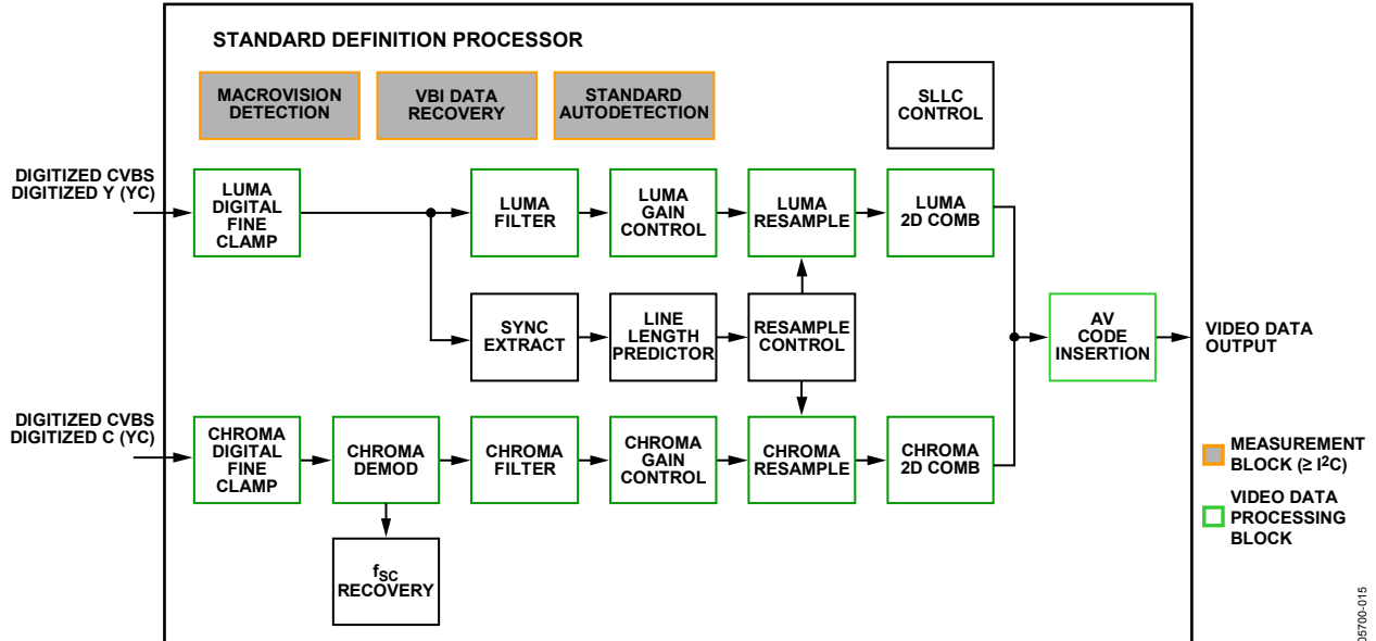
Figure 14. Block Diagram of the Video Processor
