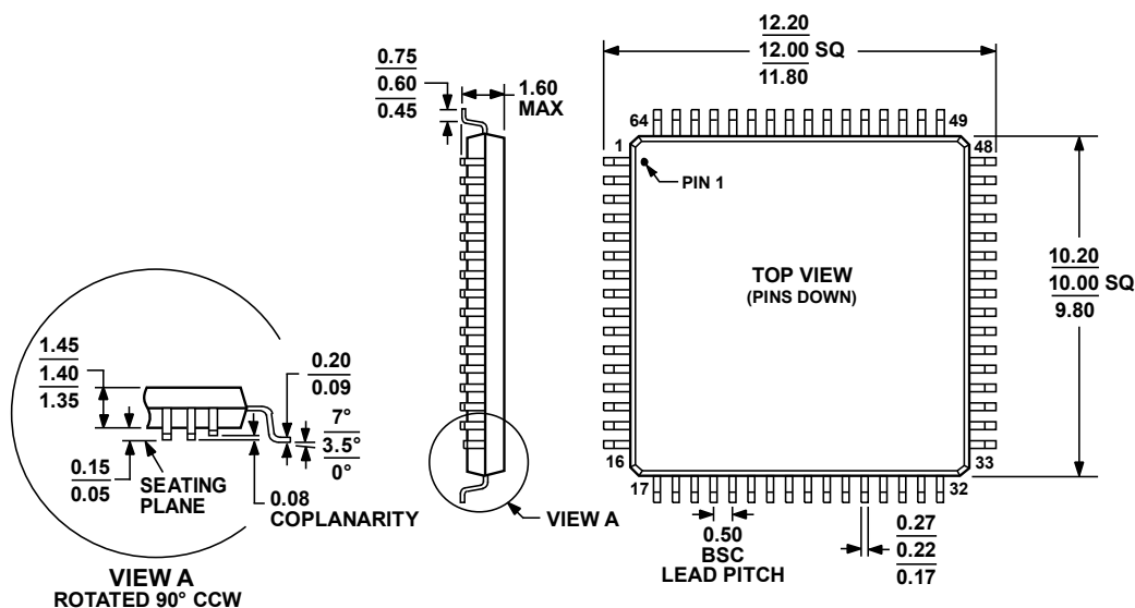
Figure 55. 64-Lead Low Profile Quad Flat Package [LQFP] 10 mm x 10 mm Body (ST-64-2) Dimensions shown in millimeters
