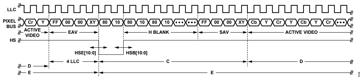
Figure 31. HS Timing
