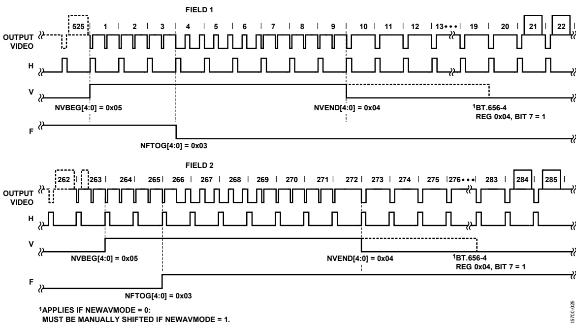
Figure 32. NTSC Default, ITU-R BT.656 (the Polarity of H, V, and F is Embedded in the Data)
