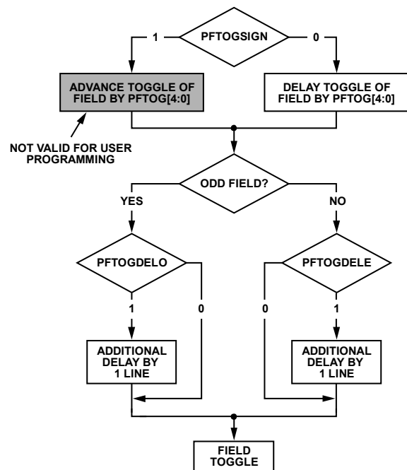
Figure 41. PAL F Toggle
