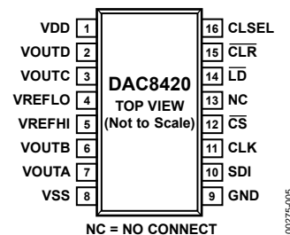
Figure 5. SOIC
