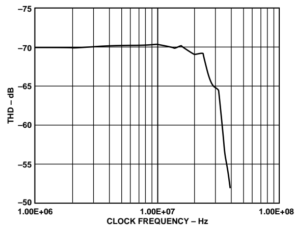
Figure 9. THD vs. Clock Frequency ( f_{IN} = 1 \text{ MHz} )
