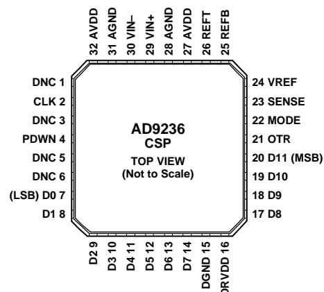
Figure 4. 32-Lead LFCSP
