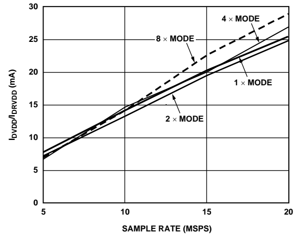
Figure 72. I_{DVDD}/I_{DRVDD} vs. Sample Rate ( DVDD = DRVDD = 5V , f_{IN} = 1\text{ MHz} )
