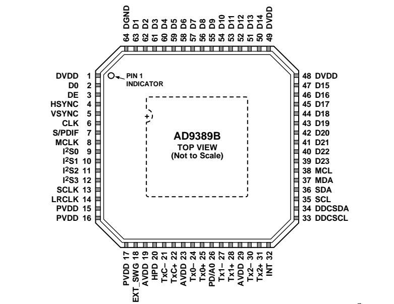
Figure 2. 64-Lead LFCSP Pin Configuration (Top View)
