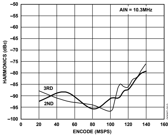
Figure 6. Second-Order and Third-Order Harmonics vs. f_{IN} , f_{IN} = 10.3 \text{ MHz}
