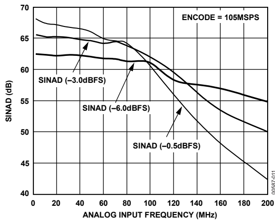
Figure 7. SINAD vs. f_{IN} , f_S = 105 \text{ MSPS}
