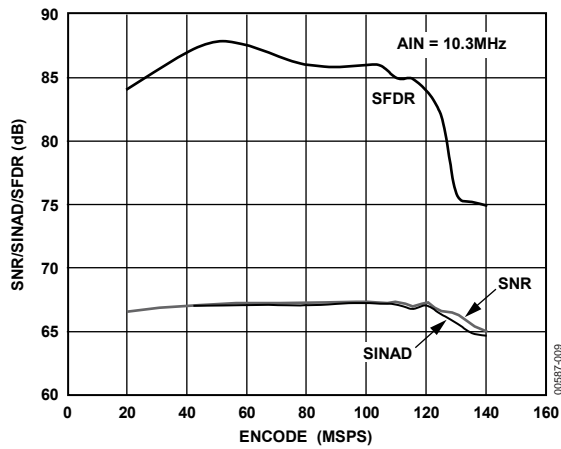
Figure 5. SNR/SINAD/SFDR vs. f_{IN} , f_{IN} = 10.3 \text{ MHz}
