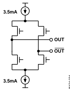
Figure 59. LVDS Output Simplified Equivalent Circuit with 3.5 mA Typical Current Source
