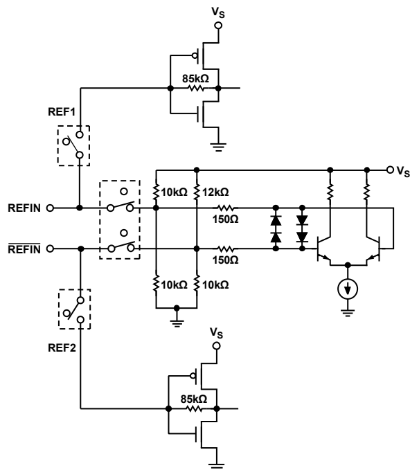
Figure 33. REF IN Equivalent Circuit
