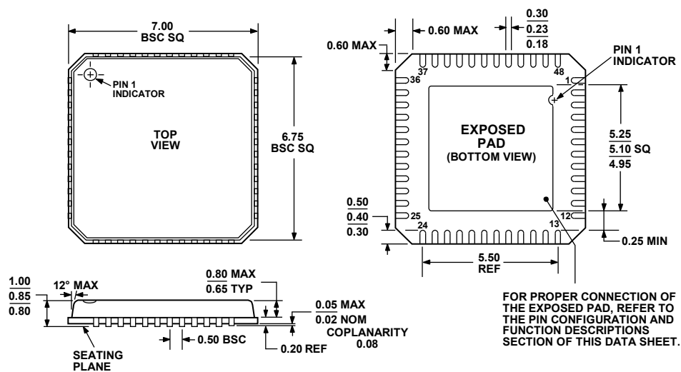
COMPLIANT TO JEDEC STANDARDS MO-220-VKGD-2 Figure 56. 48-Lead Lead Frame Chip Scale Package [LFCSP_VQ] 7 mm x 7 mm Body, Very Thin Quad (CP-48-1) Dimensions shown in millimeters
