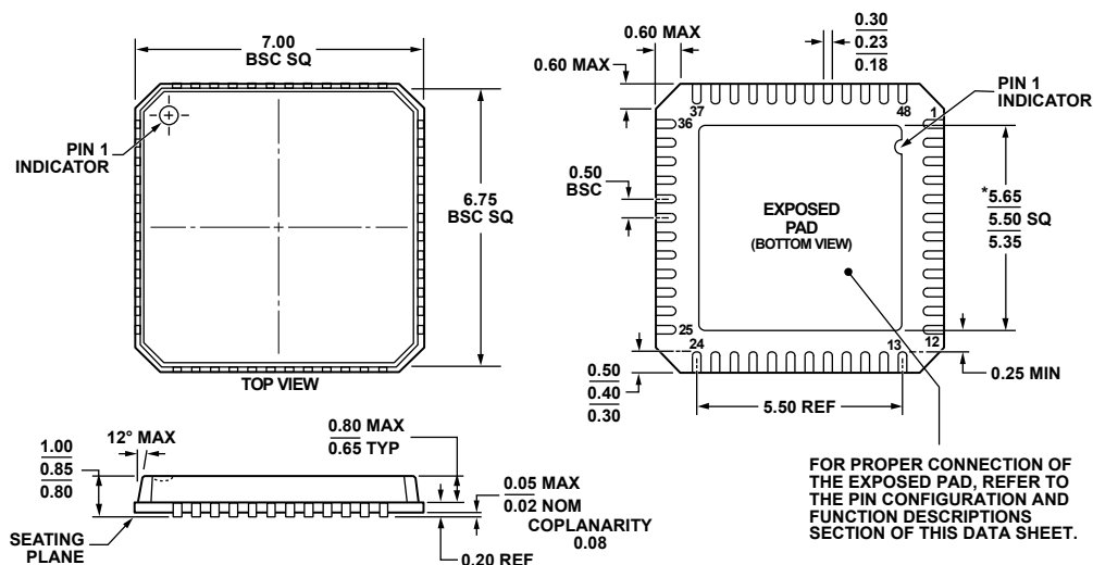
*COMPLIANT TO JEDEC STANDARDS MO-220-VKGD-2 WITH EXCEPTION TO EXPOSED PAD DIMENSION. Figure 55. 48-Lead Lead Frame Chip Scale Package [LFCSP_VQ] 7 mm x 7 mm Body, Very Thin Quad (CP-48-8) Dimensions shown in millimeters
