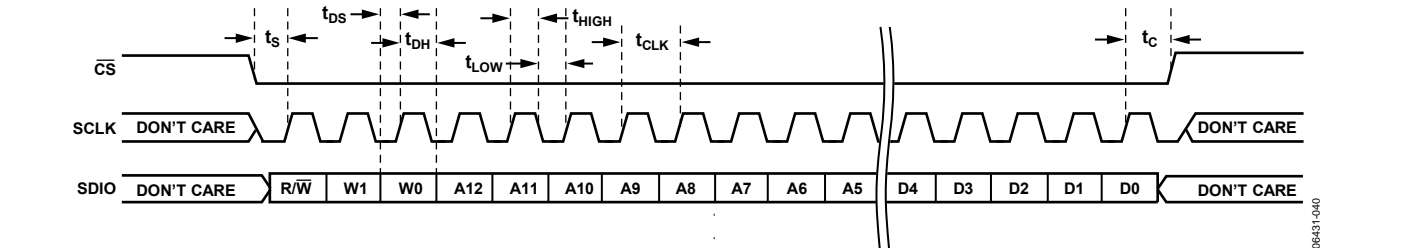
Figure 47. Serial Control Port Write—MSB First, 16-Bit Instruction, Timing Measurements
