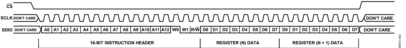
Figure 49. Serial Control Port Write—LSB First, 16-Bit Instruction, Two Bytes Data
