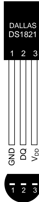
(BOTTOM VIEW)
