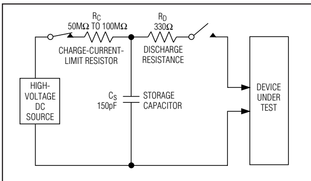
Figure 10c. IEC 1000-4-2 ESD Test Model
