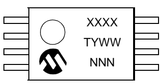
8-Lead TSSOP
