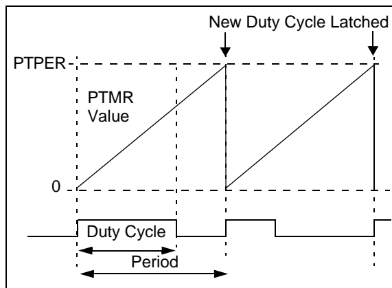
FIGURE 15-2: EDGE-ALIGNED PWM
