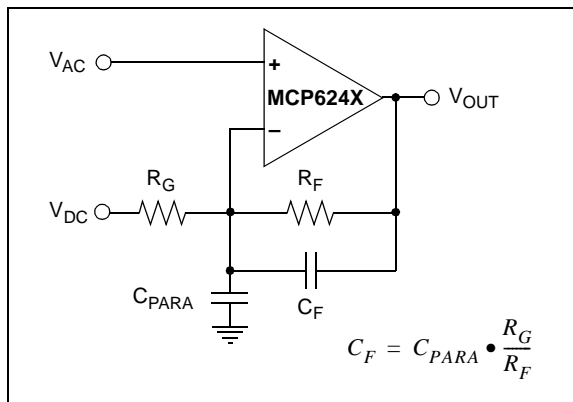
FIGURE 4-8: Effect of Parasitic Capacitance at the Input.
