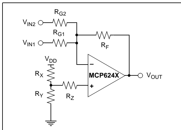
FIGURE 4-7: Summing Amplifier Circuit.
