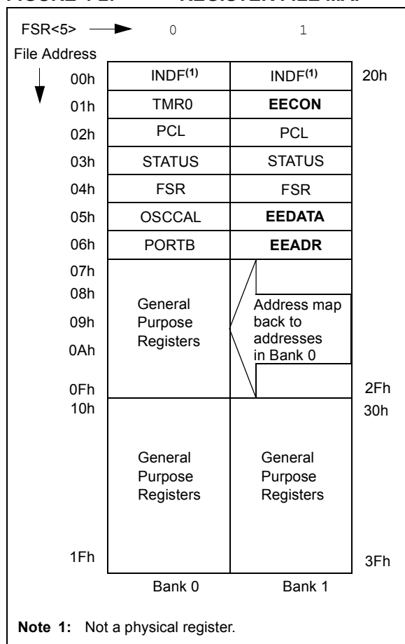
FIGURE 4-2: REGISTER FILE MAP
