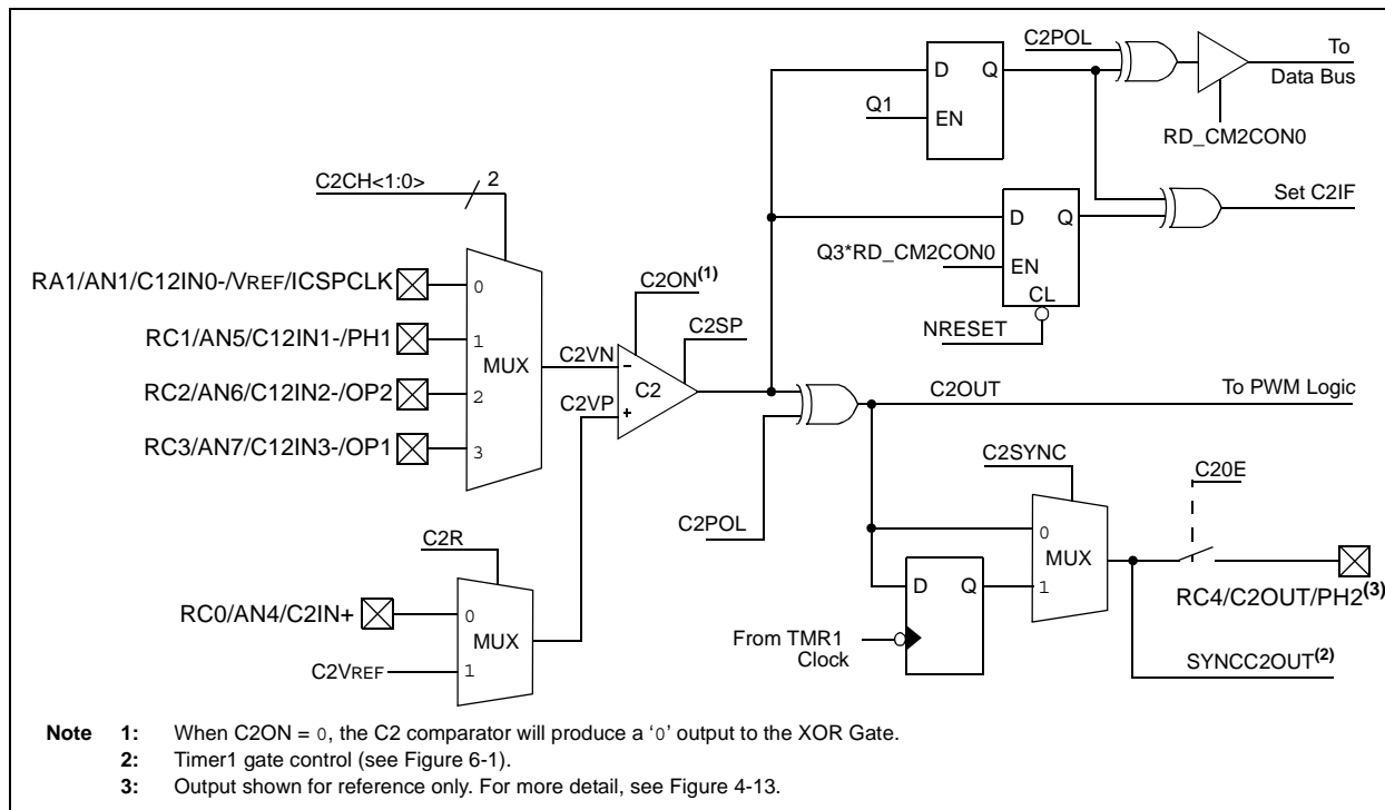
FIGURE 9-2: COMPARATOR C2 SIMPLIFIED BLOCK DIAGRAM
