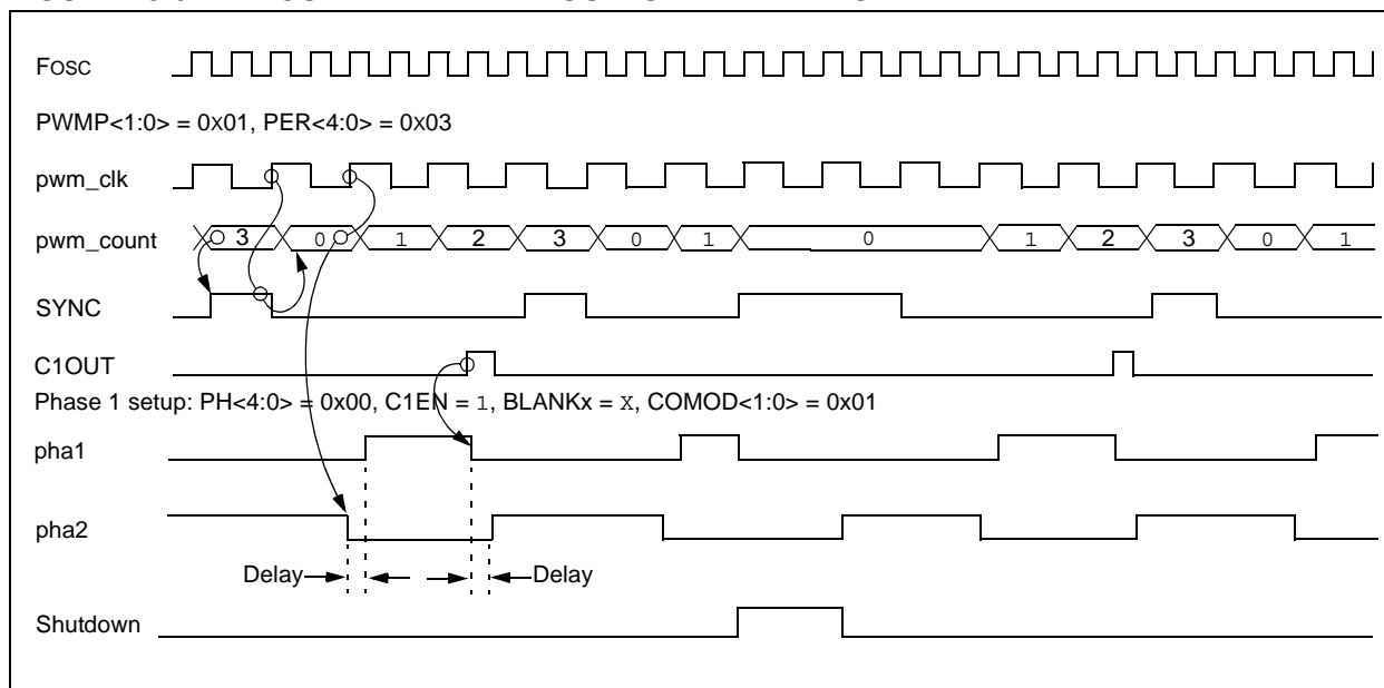
FIGURE 13-6: COMPLEMENTARY OUTPUT PWM TIMING
