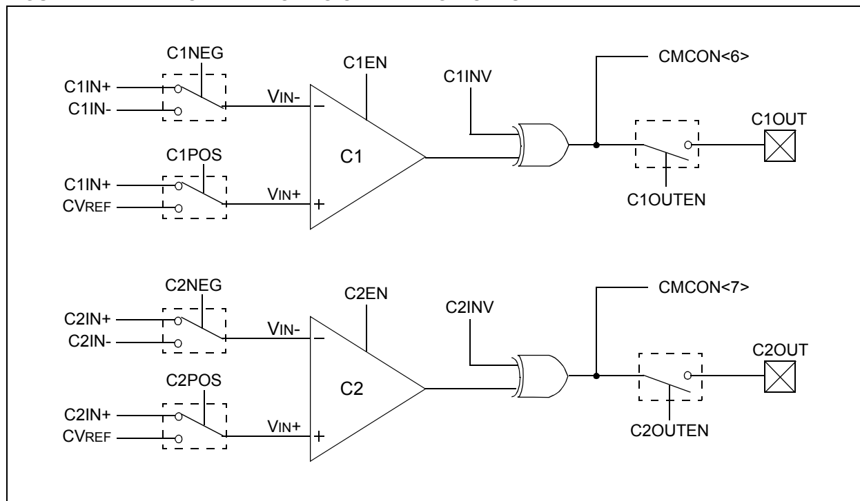
FIGURE 21-1: COMPARATOR I/O OPERATING MODES
