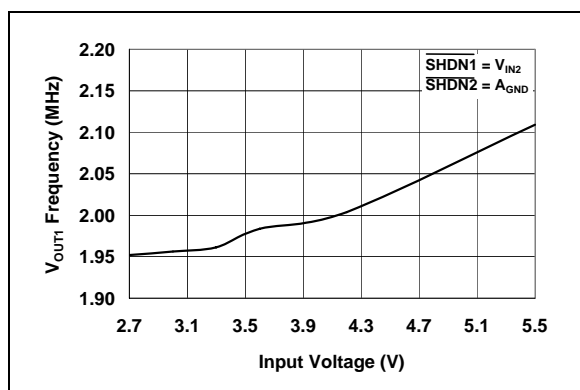
FIGURE 2-14: V_{OUT1} Switching Frequency vs. Input Voltage.
