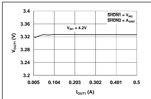
FIGURE 2-13: V_{OUT1} vs. I_{OUT1} ( V_{OUT1} = 3.3V ).
