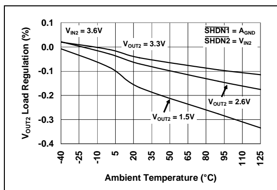
FIGURE 2-29: V_{OUT2} Load Regulation vs. Ambient Temperature.
