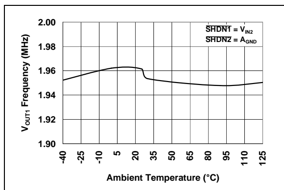
FIGURE 2-15: V_{OUT1} Switching Frequency vs. Ambient Temperature.
