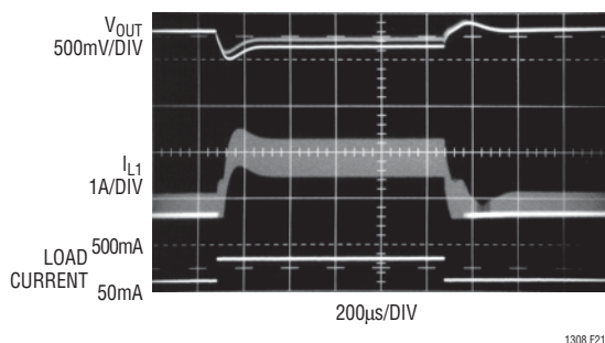
Figure 21. Load Step Response with 47 \mu F Tantalum Output Capacitor and Phase Lead Capacitor C_{PL}
