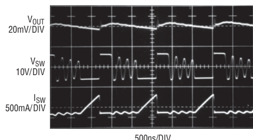
Figure 5. Converter Waveforms in Discontinuous Mode
