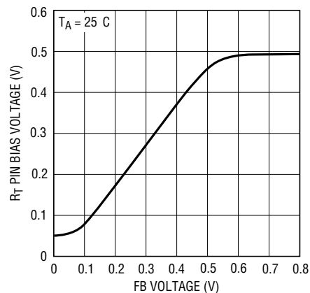
Frequency Foldback, R_T = 75.0k
