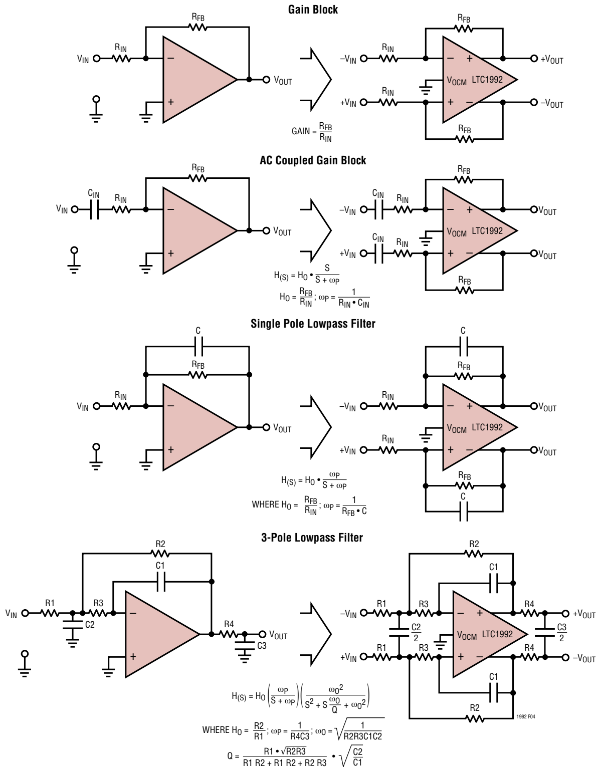
Figure 4. Basic Fully Differential Amplifier Application Circuits (Note: Single-Ended to Differential Conversion is Easily Accomplished by Connecting One of the Input Nodes, +VIN or -VIN, to a DC Reference Level (e.g., Ground))
