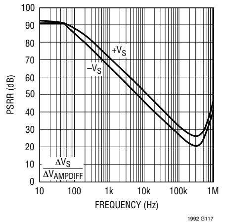
Power Supply Rejection Ratio vs Frequency (Note 7)
