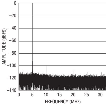
LTC2205: 64K Point FFT, 65Mps, f_{IN} = 70.1\text{MHz} , -1\text{dBFS} , PGA = 0, DITH = 0
