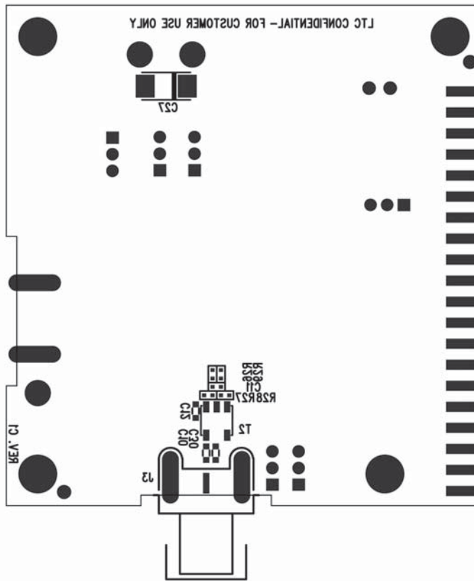
Silkscreen Bottom
