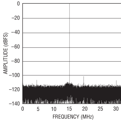
LTC2205: 64K Point FFT, 65Mps, f_{IN} = 15.1\text{MHz} , -40\text{dBFS} , PGA = 0, DITH = 0
