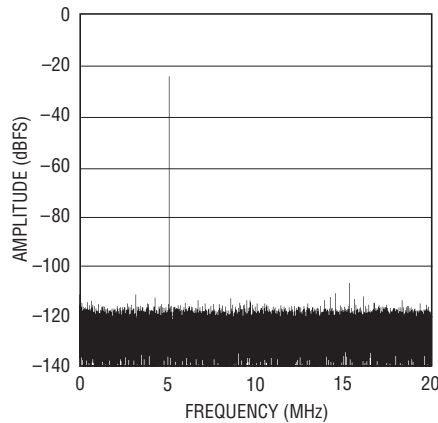
LTC2204: 64K Point FFT, 40Msps, f_{IN} = 5.1\text{MHz} , -25\text{dBFS} , \text{PGA} = 0 , \text{DITH} = 0
