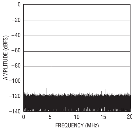
LTC2204: 64K Point FFT, 40Msps, f_{IN} = 5.1\text{MHz} , -40\text{dBFS} , \text{PGA} = 0 , \text{DITH} = 0
