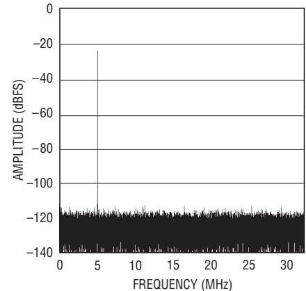
LTC2205: 64K Point FFT, 65Mps, f_{IN} = 70.1\text{MHz} , -25\text{dBFS} , PGA = 0, DITH = 0
