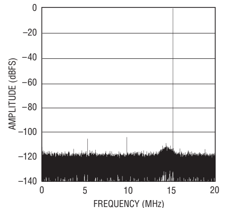
LTC2204: 64K Point FFT, 40Msps, f_{IN} = 15.1\text{MHz} , -1\text{dBFS} , \text{PGA} = 0 , \text{DITH} = 0
