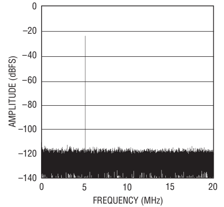
LTC2204: 64K Point FFT, 40Msps, f_{IN} = 5.1\text{MHz} , -25\text{dBFS} , \text{PGA} = 0 , \text{DITH} = 1
