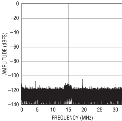
LTC2205: 64K Point FFT, 65Mps, f_{IN} = 15.1\text{MHz} , -25\text{dBFS} , PGA = 0, DITH = 1
