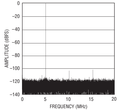
LTC2204: 64K Point FFT, 40Msps, f_{IN} = 5.1\text{MHz} , -1\text{dBFS} , \text{PGA} = 0 , \text{DITH} = 0
