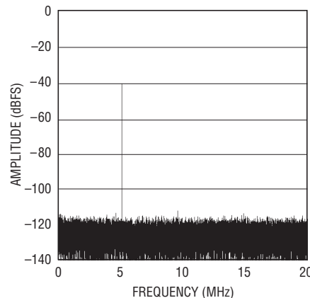
LTC2204: 64K Point FFT, 40Msps, f_{IN} = 5.1\text{MHz} , -40\text{dBFS} , \text{PGA} = 0 , \text{DITH} = 1
