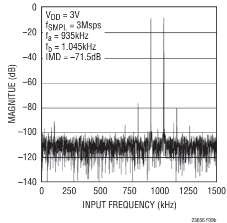
Figure 9b. LTC2366 Intermodulation Distortion Plot
