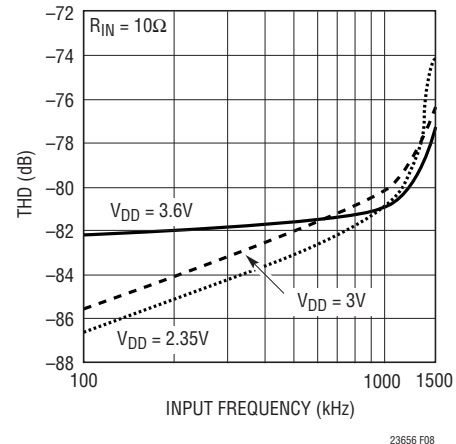
Figure 8. LTC2366 Distortion vs Input Frequency
