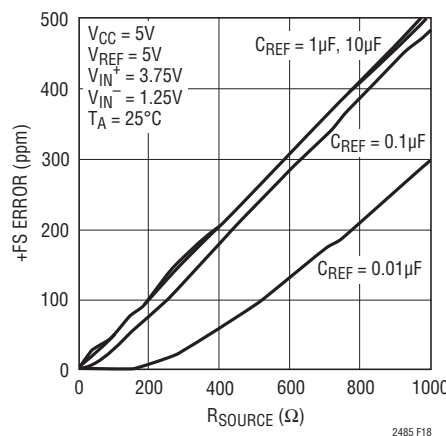
Figure 18. +FS Error vs R_{SOURCE} at REF+ or REF- (Large C_{REF} )
