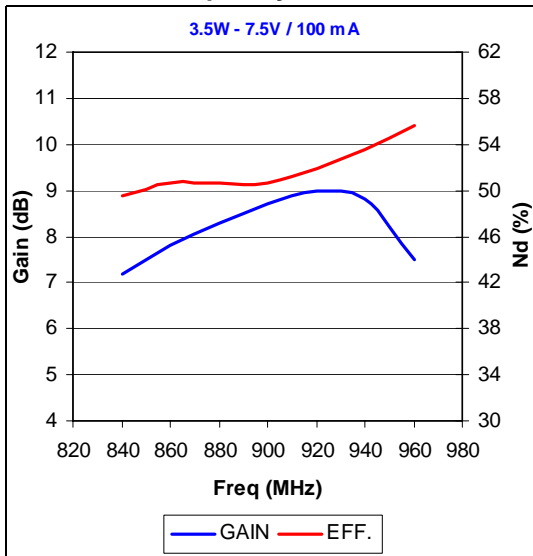
Figure 3. Gain and efficiency vs frequency
