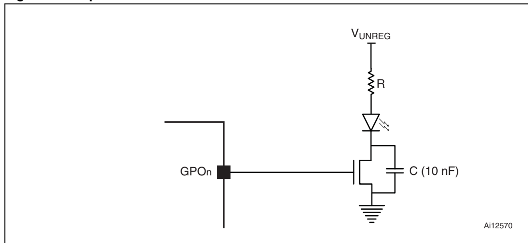
Figure 5. Optional LED schematic
