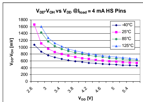
Figure 18. Typical V_{DD}-V_{OH} vs. V_{DD} at I_{load} = 4\text{ mA}
