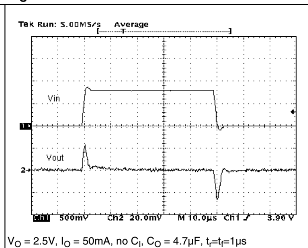
Figure 14. Line transient
