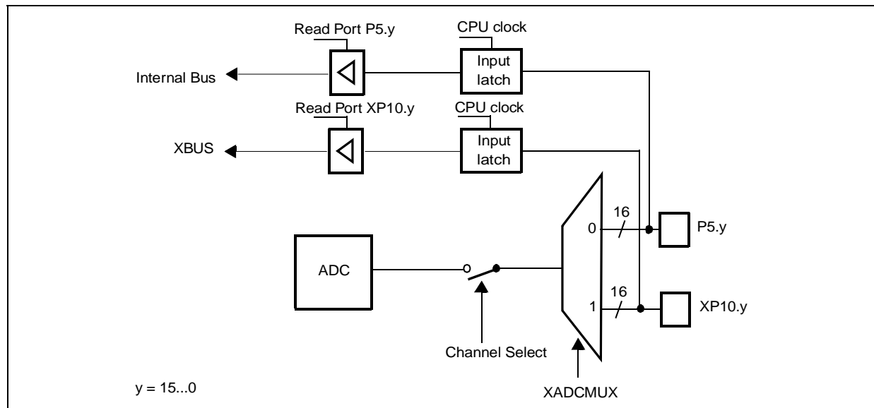
Figure 52 : Block Diagram
