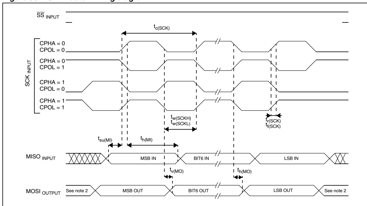
Figure 83. SPI master timing diagram (1)
